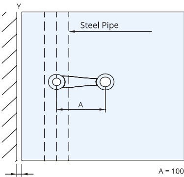
Glass Preparation for Front Glass :
