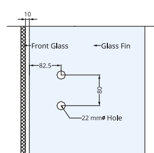
Articulated Bolts
