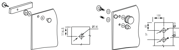
Guide Rail Installation Diagram
