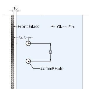
Fixed Bolts
